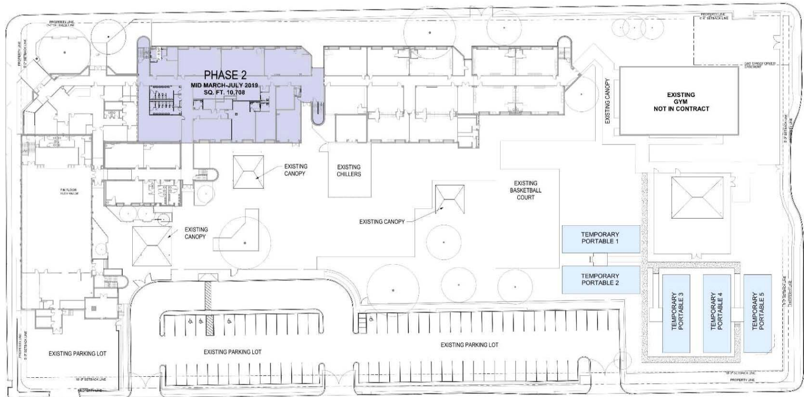
First Floor
